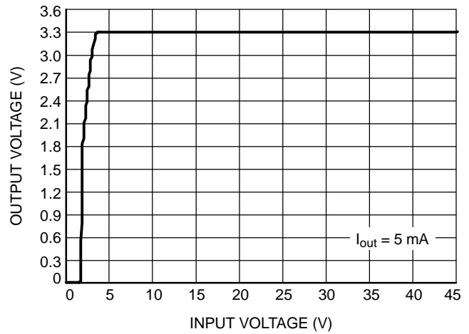
Figure 12. Input Voltage vs. Output Voltage (3.3 V Version)
