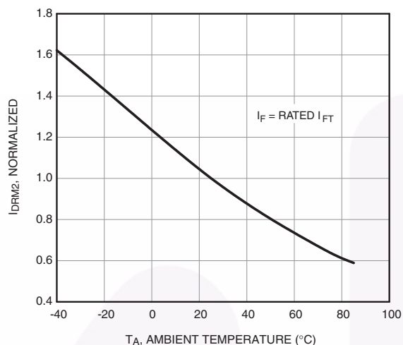
Figure 5. I_{\text{DRM2}} - Leakage in Inhibit State vs. Temperature
