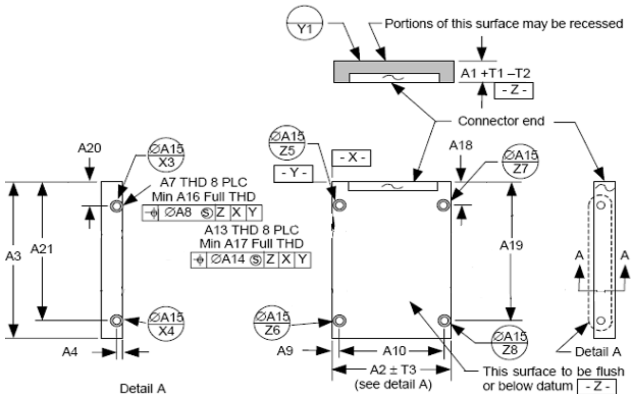
Figure 5: Housing dimensions
