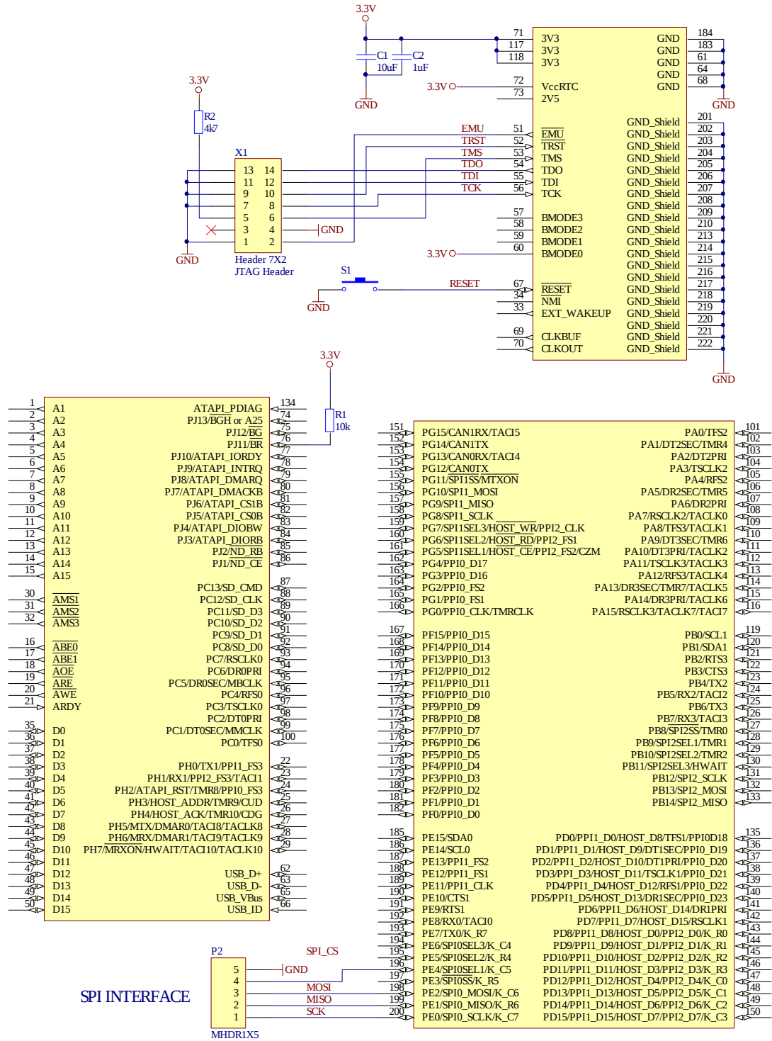
Figure 5-1: Schematic
