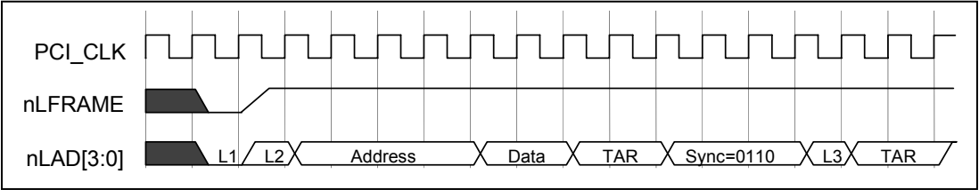
FIGURE 12 – I/O WRITE
