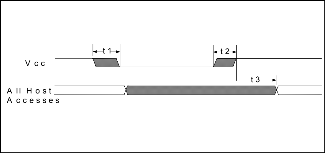
FIGURE 8 - POWER-UP TIMING
