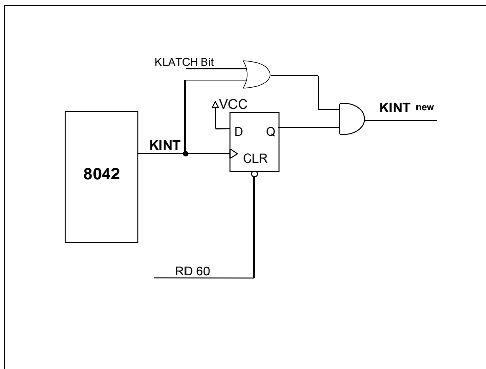
FIGURE 5 – KEYBOARD LATCH
