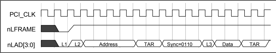
FIGURE 13 – I/O READ
