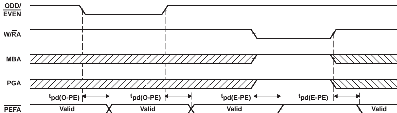
Figure 16. ODD/ \overline{\text{EVEN}} , \text{W}/\overline{\text{RA}} , MBA, and PGA to \overline{\text{PEFA}} Timing
