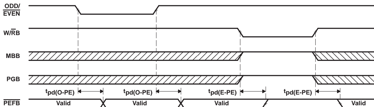
Figure 17. ODD/ \overline{\text{EVEN}} , \text{W}/\overline{\text{RB}} , MBB, and PGB to \overline{\text{PEFB}} Timing
