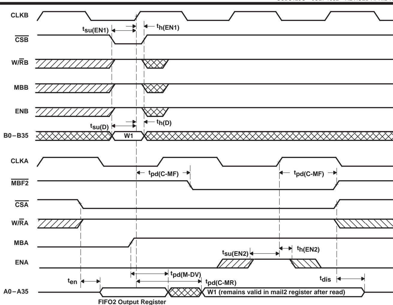
Figure 15. Timing for Mail2 Register and MBF2 Flag
