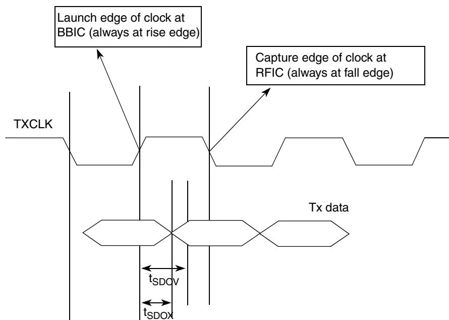
Figure 43. RF Serial Interface AC Timing Diagram
