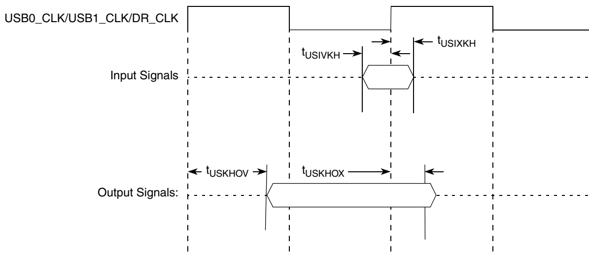
Figure 24. USB Signals
