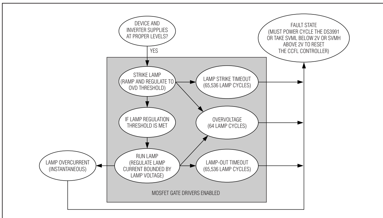
Figure 3. Fault-Handling Flowchart
