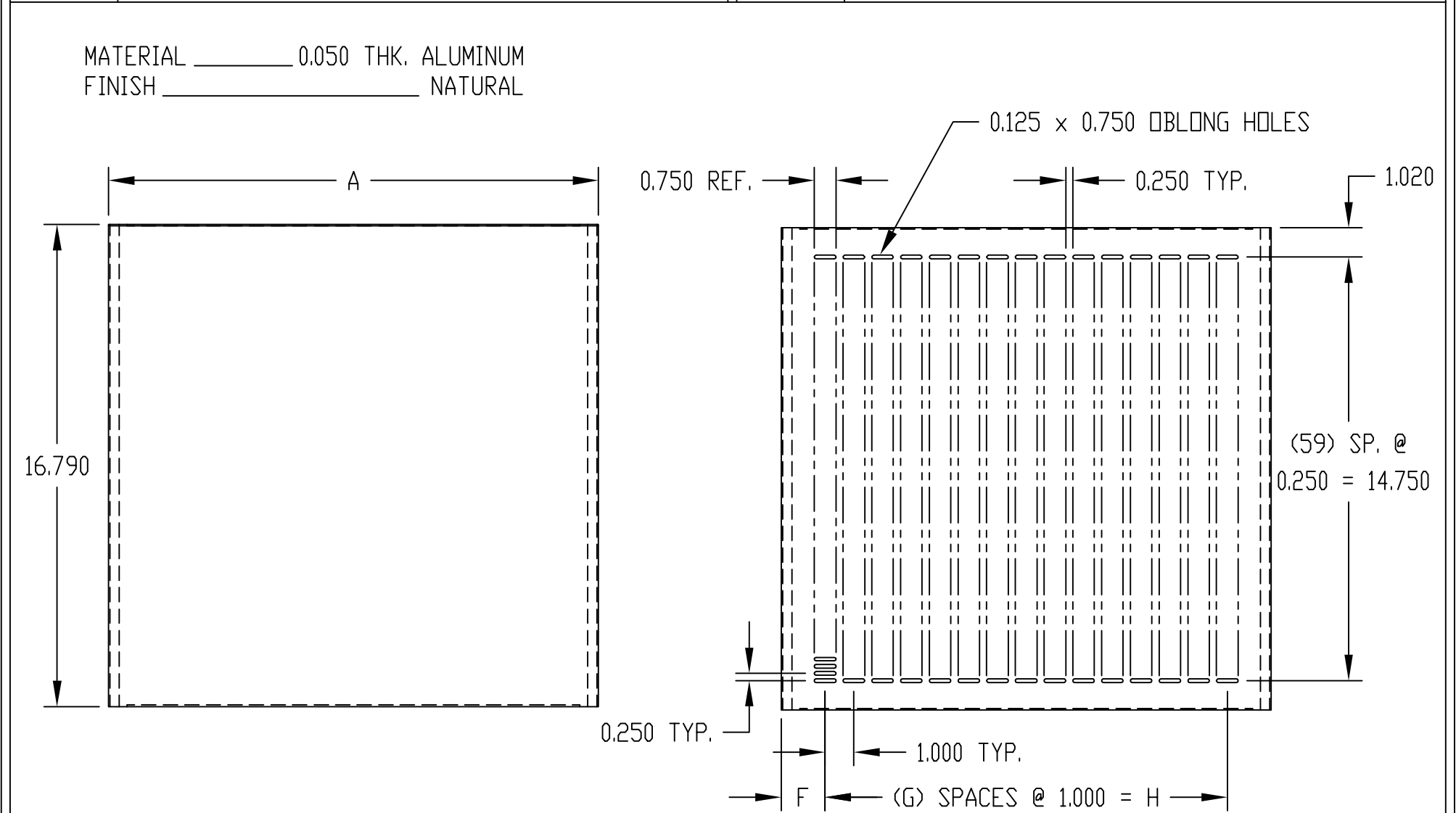
SOLID TOP OR BOTTOM COVER TBC-14252 & TBC-14253
