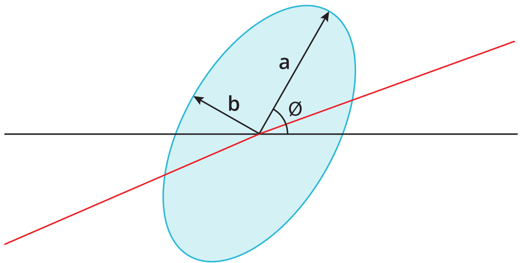
Figure 7. 3- and 5-step MacAdam ellipse illustration for Tables 8a-8h.
