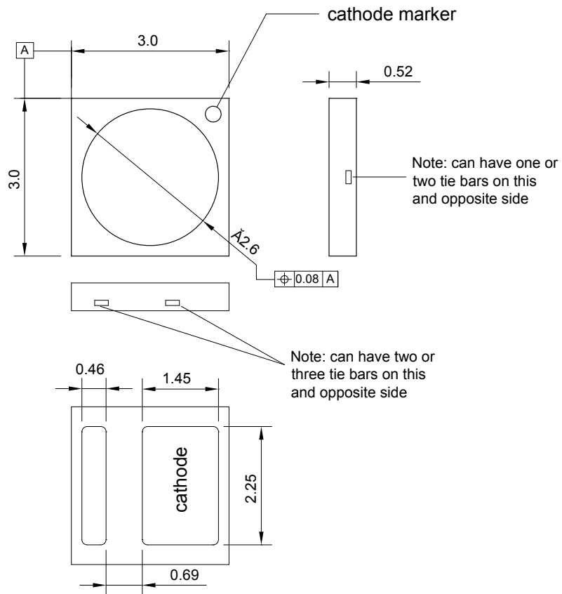
Figure 9. Mechanical dimensions for LUXEON 3030 2D.
