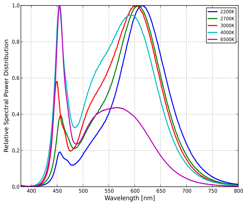
Figure 1b. Typical normalized power vs. wavelength for L130-xx80003000W21 120mA, T j =25°C.
