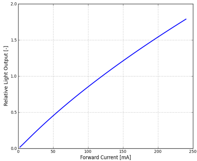
Figure 3. Typical normalized light output vs. forward current for L130-xxxx003000W21 at T_j=25^{\circ}\text{C} .
