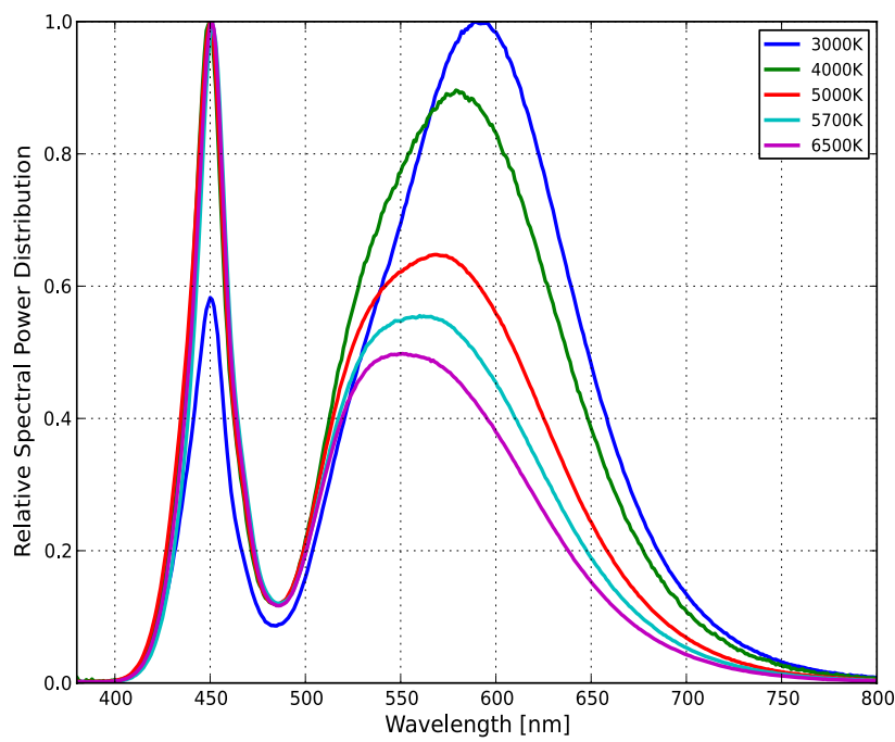
Figure 1a. Typical normalized power vs. wavelength for L130-xx70003000W21 at 120mA, T j =25°C.
