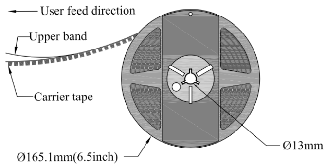
Figure 13. Reel dimensions for LUXEON 3030 2D.
