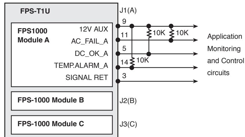
Fig 19-5 Supervisory Signals
