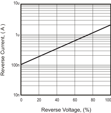
Fig.1 - Reverse Characteristics
