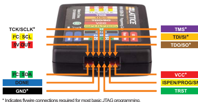
Figure 2. Programming Cable In-System Programming Interface for the PC (HW-USB-2B) 1
