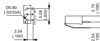
L254 Right angle, spacing 2,54 (.100)
