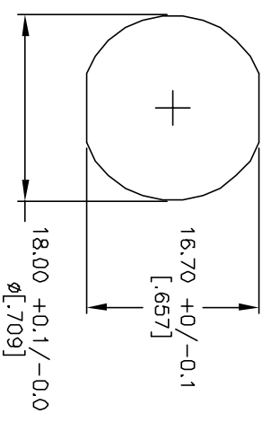
RECOMMEND PANEL MOUNTING
