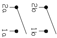
CIRCUIT: 4P, DPST CONTACT CONFIGURATION
