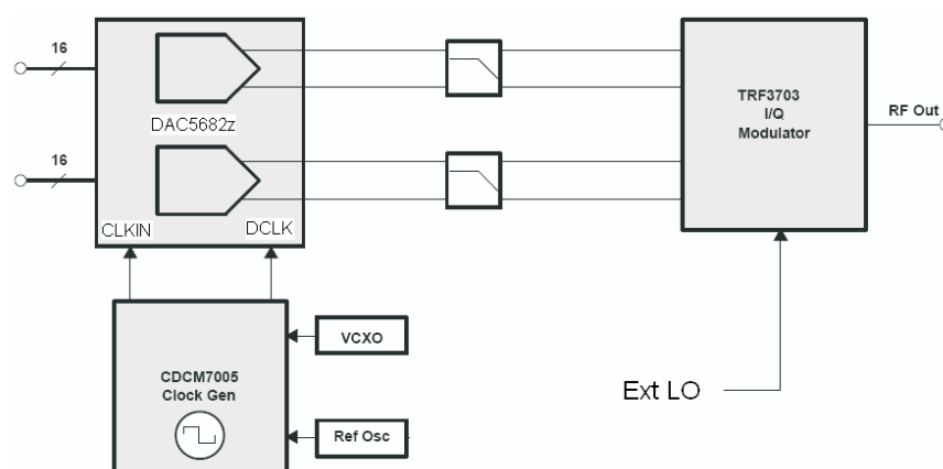
Figure 5. DAC5682z Option Block Diagram
