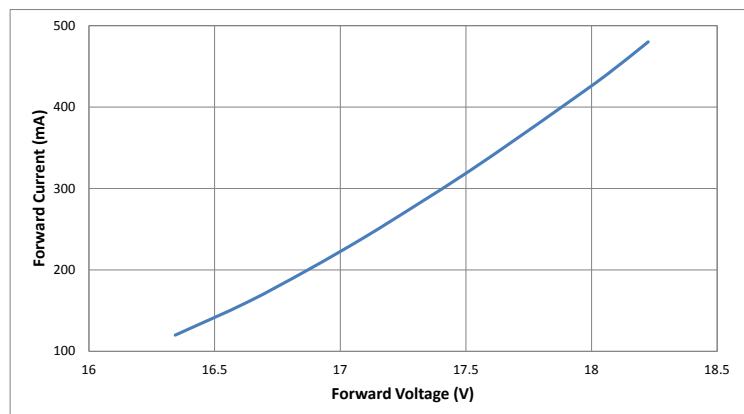
Forward Current vs. Forward Voltage @ 85°C
