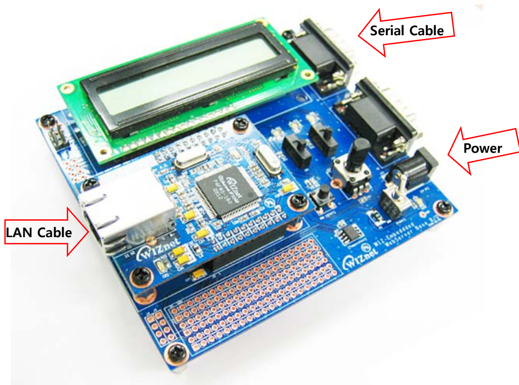
Figure 19. WIZ-Embedded WebServer External Interface
