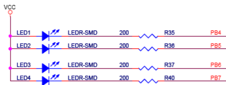
Figure 6. WIZ-Embedded WebServer LED
