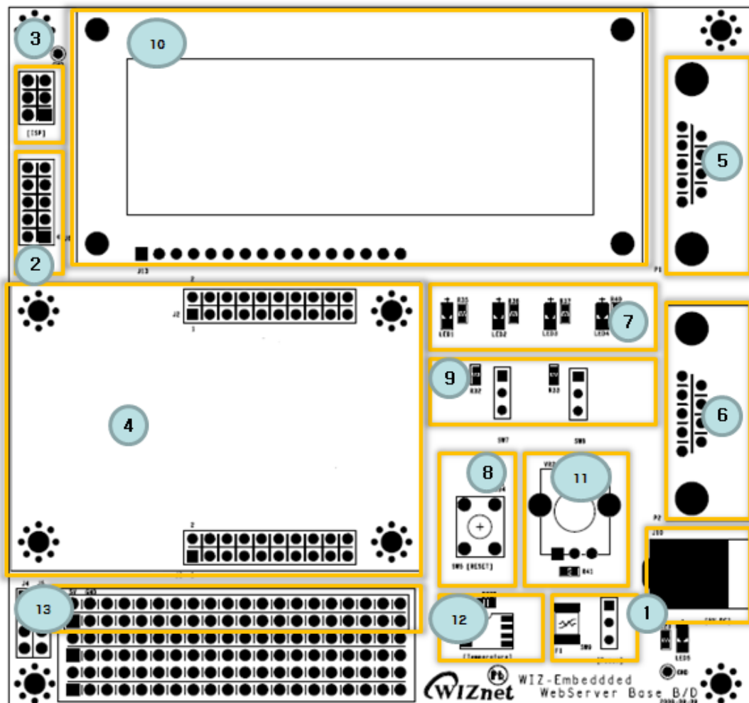
Figure 2. WIZ-Embedded WebServer Base Board Layout
