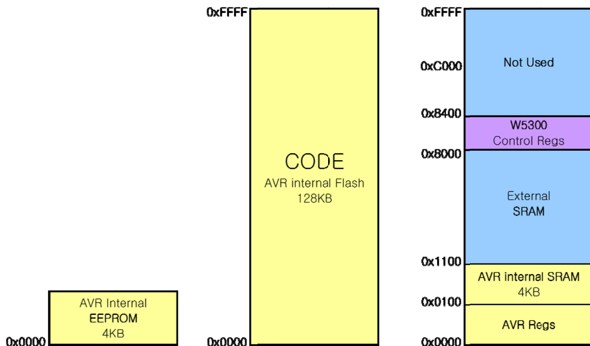
Figure 24. WIZ-Embedded WebServer Memory Map
