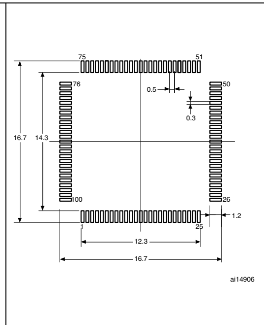
Figure 42. Recommended footprint (1)(2)
