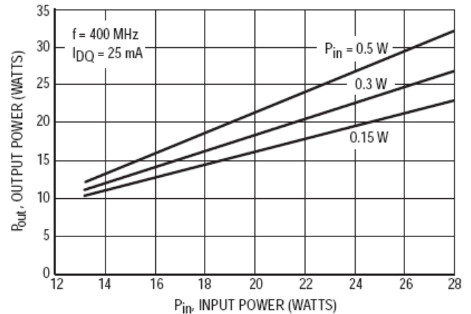
Figure 7. Output Power versus Input Power
