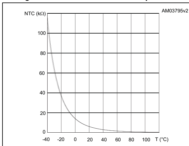
Figure 7. NTC resistance vs. temperature
