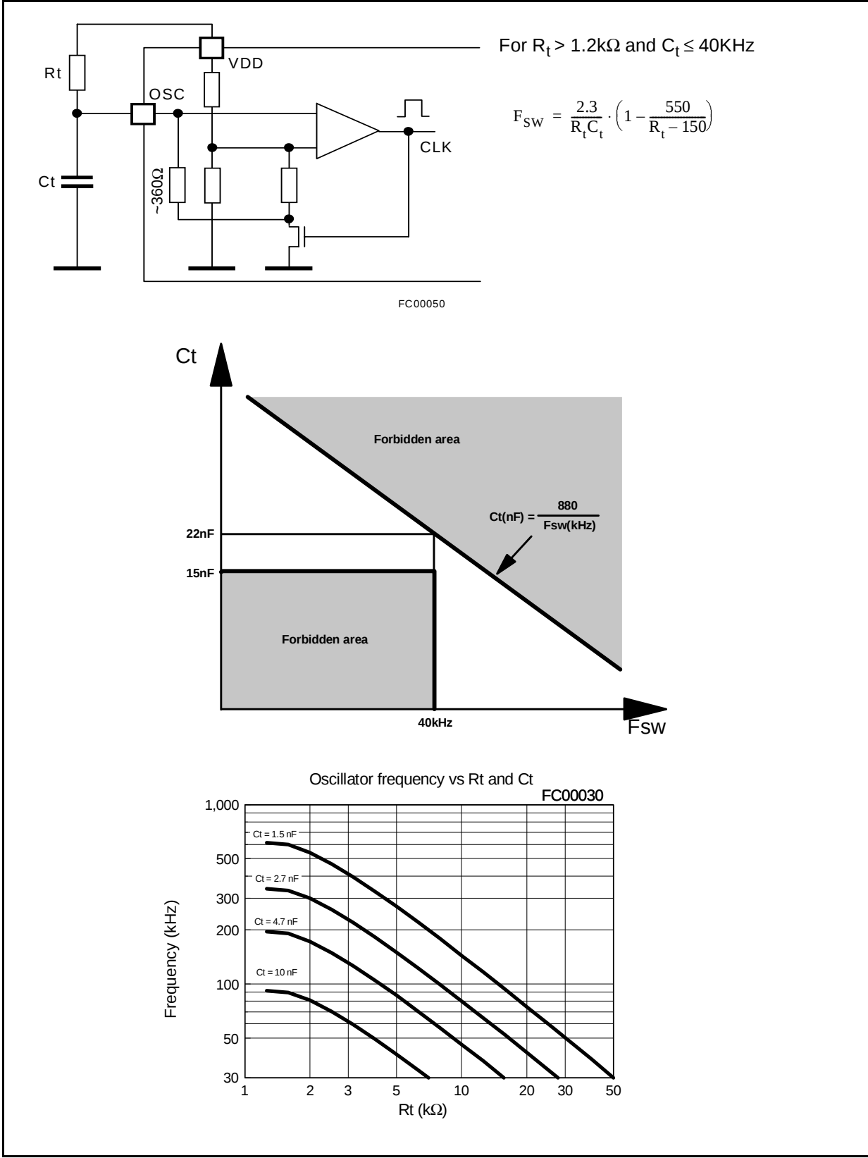
Figure 14. Oscillator
