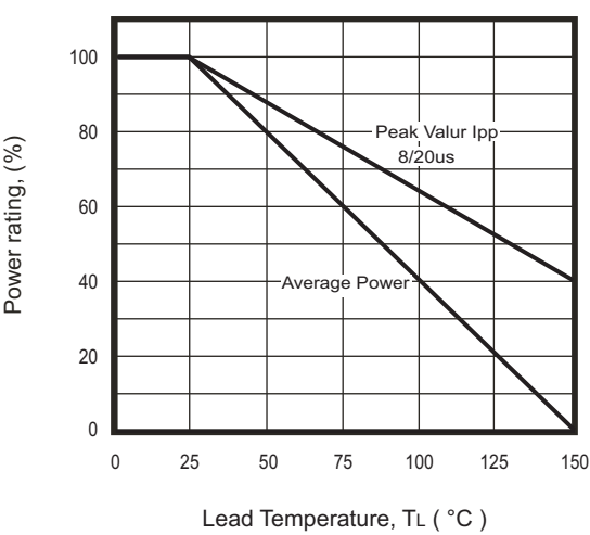
Fig. 2 - Power Derating Curve
