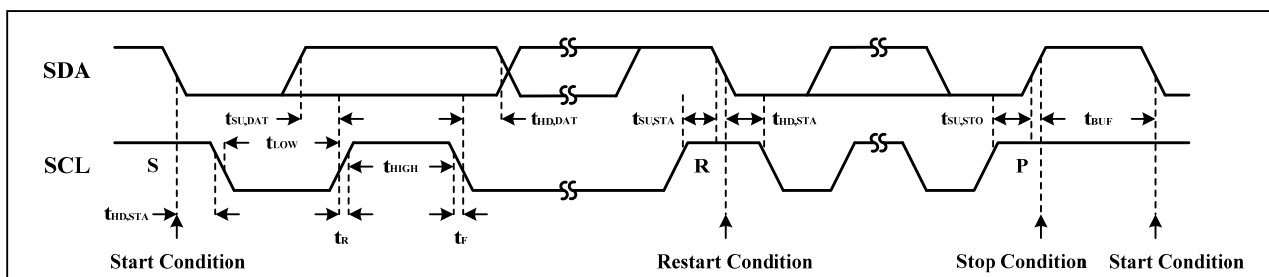
Figure 2 Interface timing
