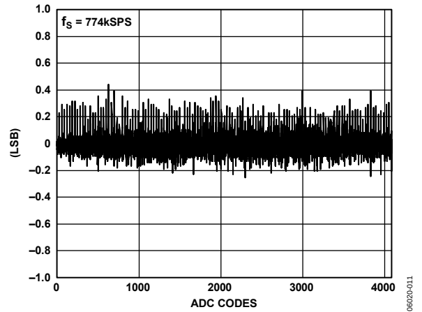
Figure 15. Typical DNL Error, f_s = 774 kSPS
