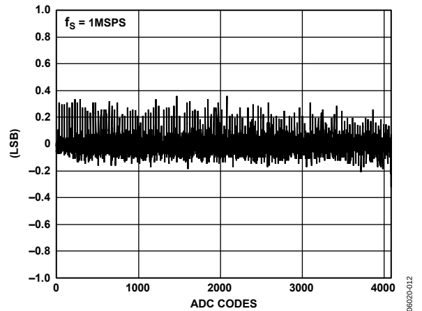
Figure 16. Typical DNL Error, f_s = 1 MSPS
