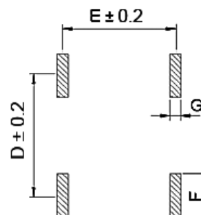
Recommended Solder Pad Layout
