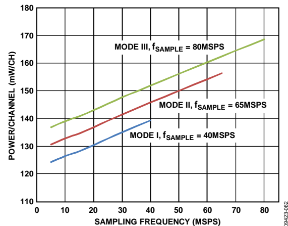
Figure 60. Power per Channel vs. f_{\text{SAMPLE}} for f_{\text{IN}} = 5 MHz
