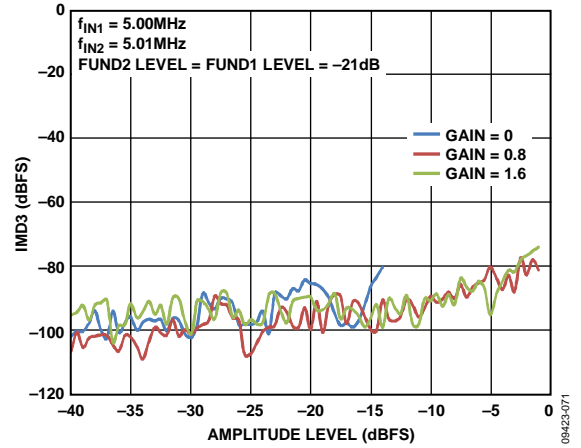
Figure 20. IMD3 vs. ADC Output Level
