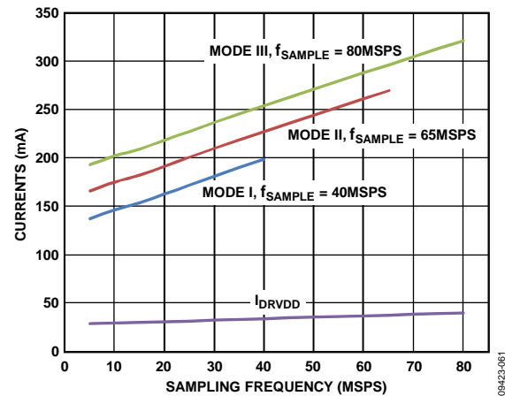
Figure 59. Supply Current vs. f_{\text{SAMPLE}} for f_{\text{IN}} = 5 MHz
