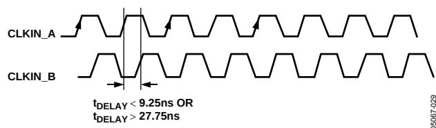
Figure 53. Clock Phase with Two Input Clocks
