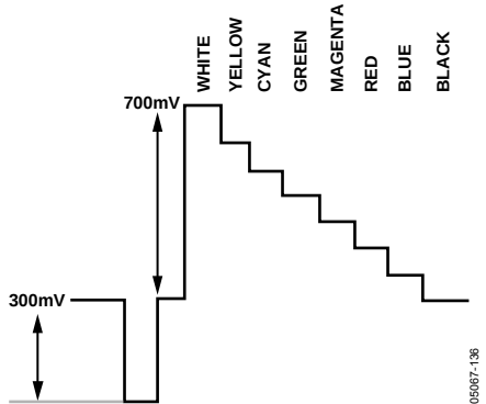
Figure 136. Y Levels—PAL
