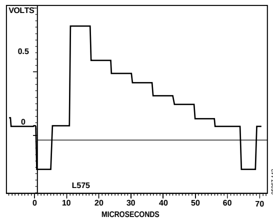
Figure 141. PAL Chroma
