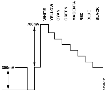
Figure 135. Y Levels—NTSC
