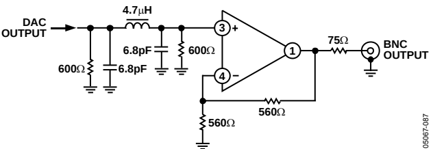
Figure 87. Example of Output Filter for PS, 8× Oversampling
