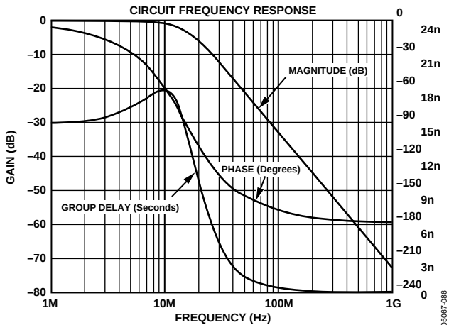
Figure 86. Filter Plot for Output Filter for SD, 16× Oversampling
