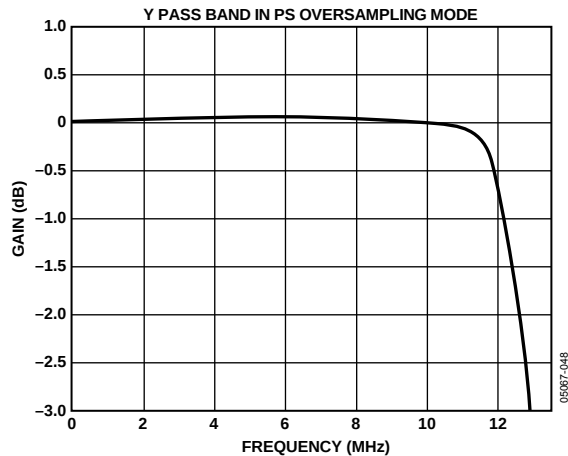
Figure 23. PS—Y 8× Oversampling Filter (Pass Band)
