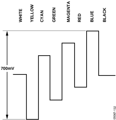
Figure 132. Pb Levels—PAL
