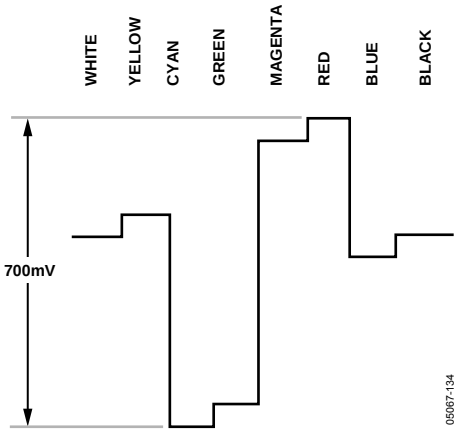
Figure 134. Pr Levels—PAL
