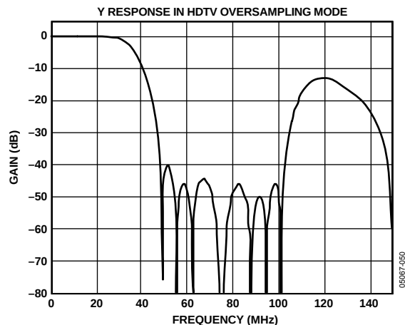
Figure 25. HDTV—Y 2× Oversampling Filter
