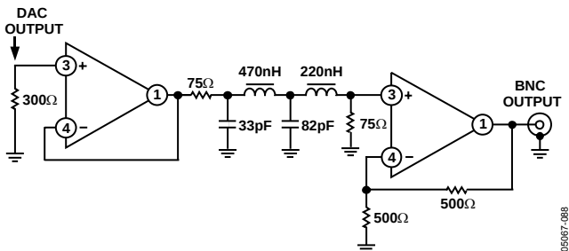
Figure 88. Example of Output Filter for HDTV, 2× Oversampling
