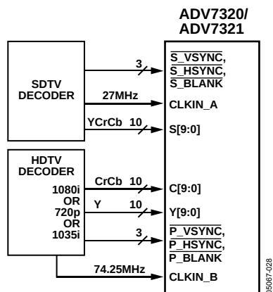
Figure 52. Simultaneous SD and HD Input
