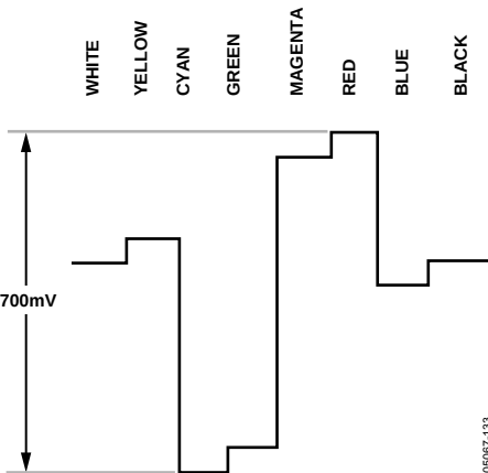
Figure 133. Pr Levels—NTSC
