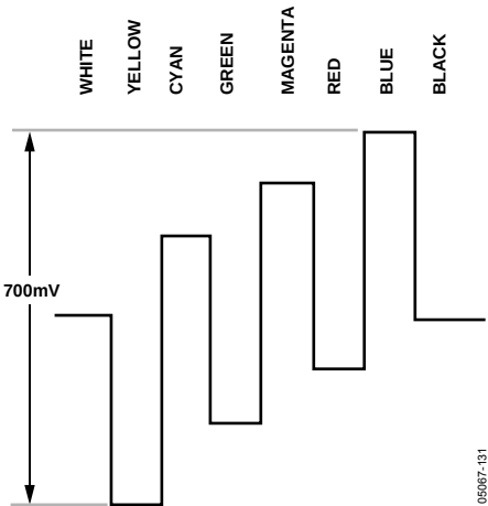
Figure 131. Pb Levels—NTSC
