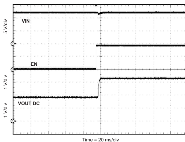
Figure 17. Prebias Start Up Relative to EN
