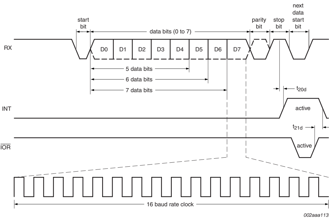
Fig 24. Receive timing
