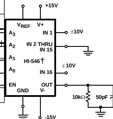
FIGURE 6B. TEST CIRCUIT
