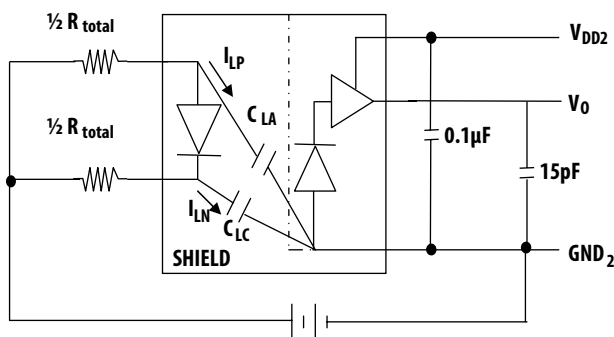
Figure 14. AC equivalent of ACPL-M75L
