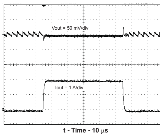
Figure 6. 1.05-V, LOAD TRANSIENT RESPONSE
