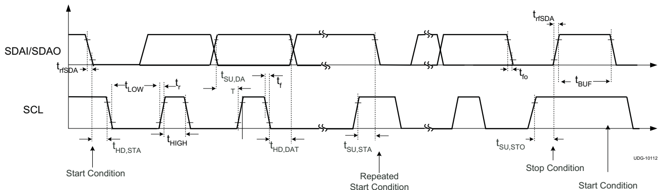
Figure 25. I²C Timings
