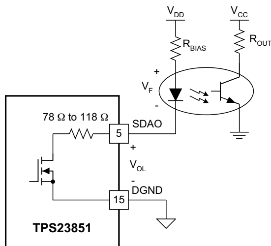
Figure 33. I 2 C Optocoupler Interface
