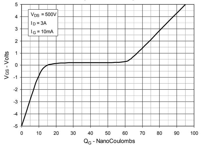
Fig. 14. Gate Charge
