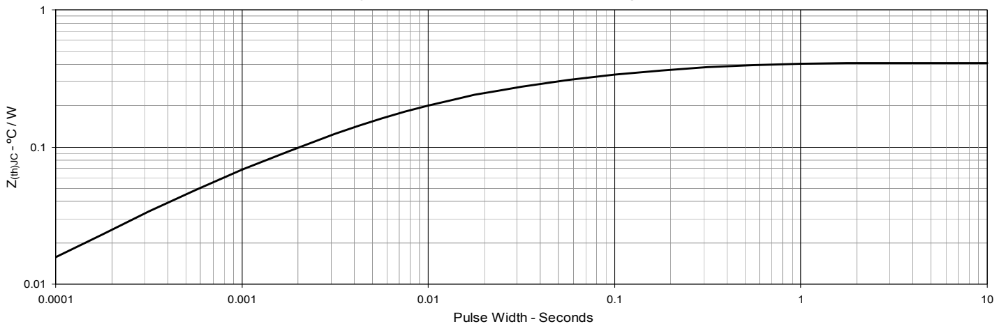
Fig. 17. Maximum Transient Thermal Impedance
