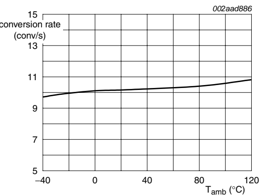
Fig 31. Conversion rate
