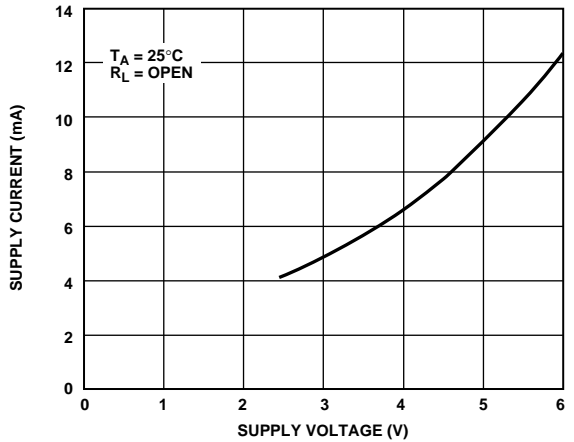
Figure 33. Supply Current vs. Supply Voltage
