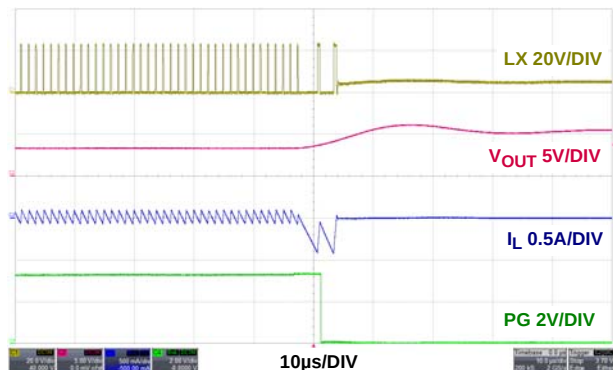
FIGURE 31. NEGATIVE CURRENT LIMIT, PWM
