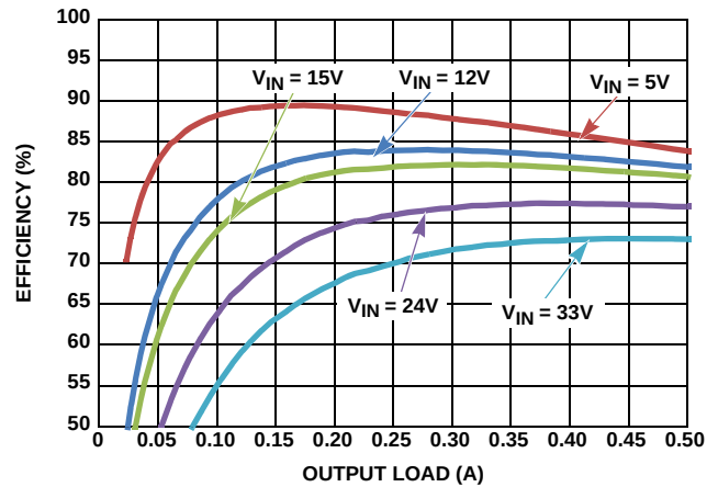
FIGURE 10. EFFICIENCY vs LOAD, PWM, V_{OUT} = 1.8\text{V}
