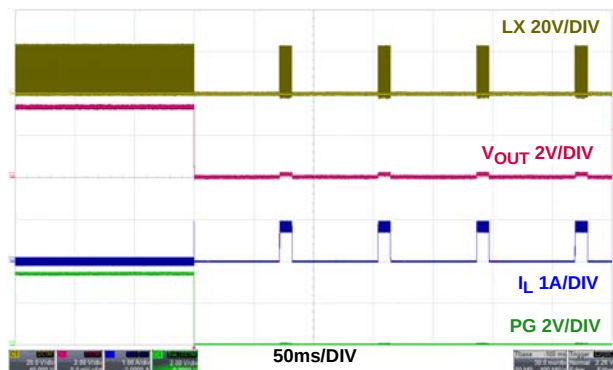
FIGURE 29. OVERCURRENT PROTECTION HICUP, PWM
