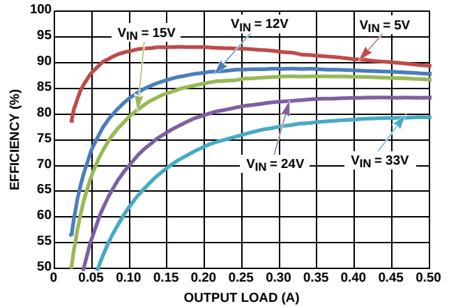
FIGURE 8. EFFICIENCY vs LOAD, PWM, V_{OUT} = 3.3\text{V}
