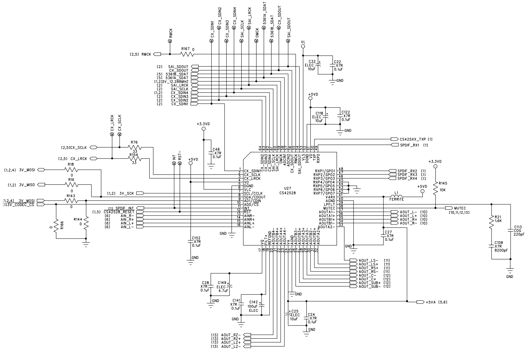
Figure 9. CoDec
