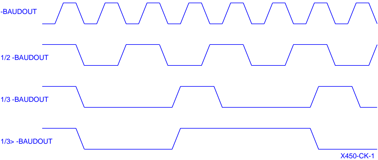
Clock timing
