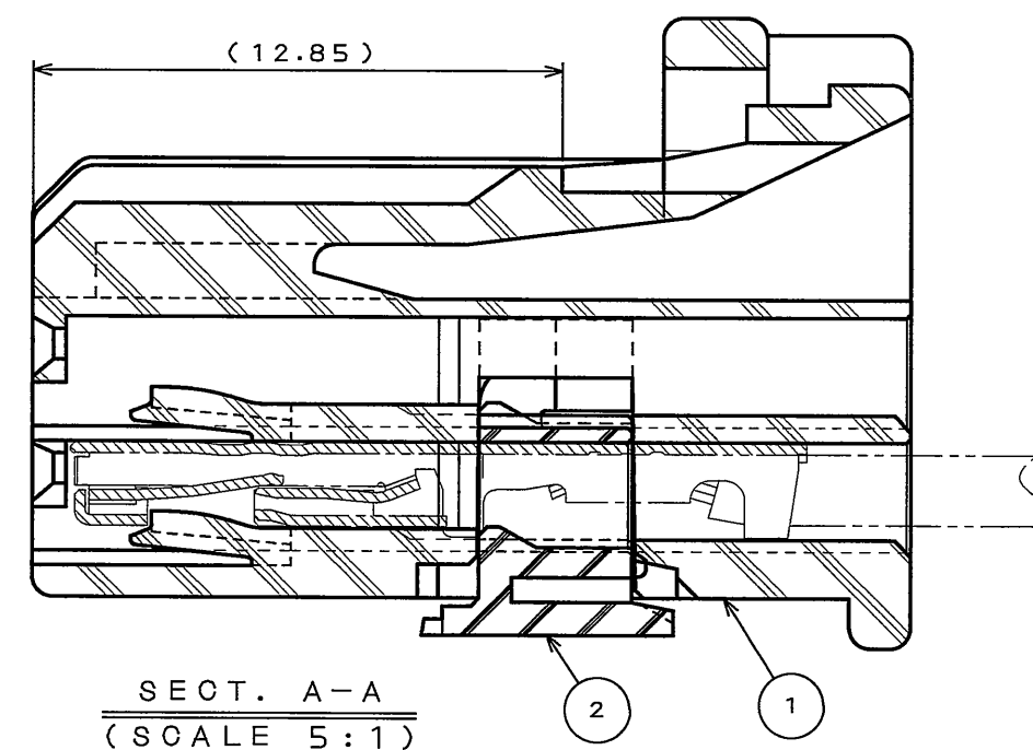
CODE PART TITLE SJ No. MATERIALS PLATING APPLICABLE WIRE S M34S75C4F1 038527 HIGH CONDUCTIVITY COPPER ALLOY TIN PLATING スズめっき CHFUS 0.22sq. AVSS 0.3sq. CHFUS 0.35sq. ALL CAVITIES CAN BE APPLIED. 全キャビティ対応 M M34S75C4F2 038528 高導電性銅合金 CHFUS 0.5sq. AVSS 0.5sq. CAVS 0.5sq. CHFS 0.75sq. CHFUS 0.75sq. ALL CAVITIES CAN BE APPLIED. 全キャビティ対応 C M34S75C4F3 038747 CAN SD 0.35sq. FOUR BOTH ENDS CAVITIES CAN BE APPLIED. 両端4箇所のカビティ対応 L M34S75C4F4 038893 AVSS 0.85sq. CAVS 0.85sq. FOUR BOTH ENDS CAVITIES CAN BE APPLIED. 両端4箇所のカビティ対応 X M34S75C4F5 109336 CHFUS 0.13sq. ALL CAVITIES CAN BE APPLIED. 全キャビティ対応
