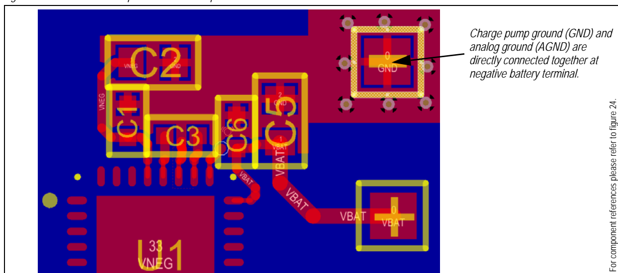
Figure 44. AS3422 Star Shaped Ground Concept
