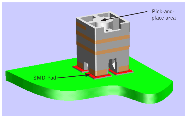
Illustration showing the 2.4GHz SMD On-ground antenna mounted onto a PCB
