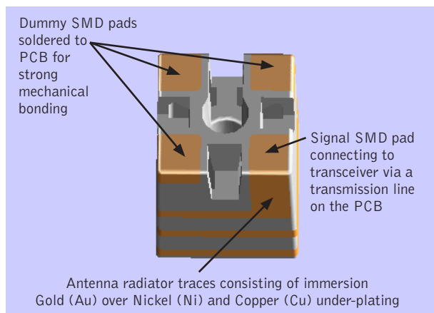
Illustration showing the plated SMD pads of the 2.4GHz SMD On-ground antenna base
