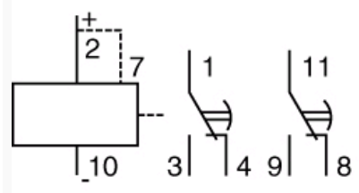
Timer 815 - 11-pin
