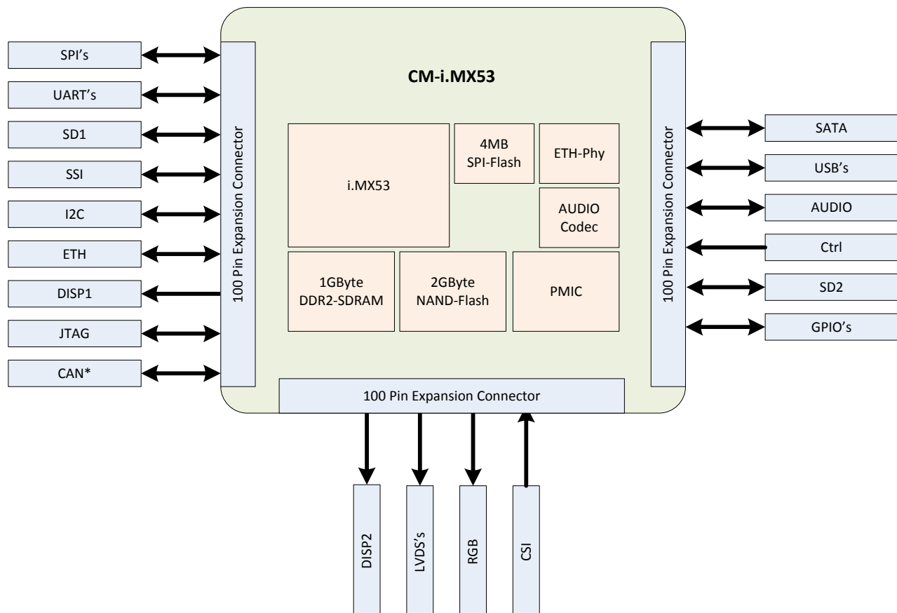
Figure 1-1: Main components of the CM-i.MX53 Core Module
