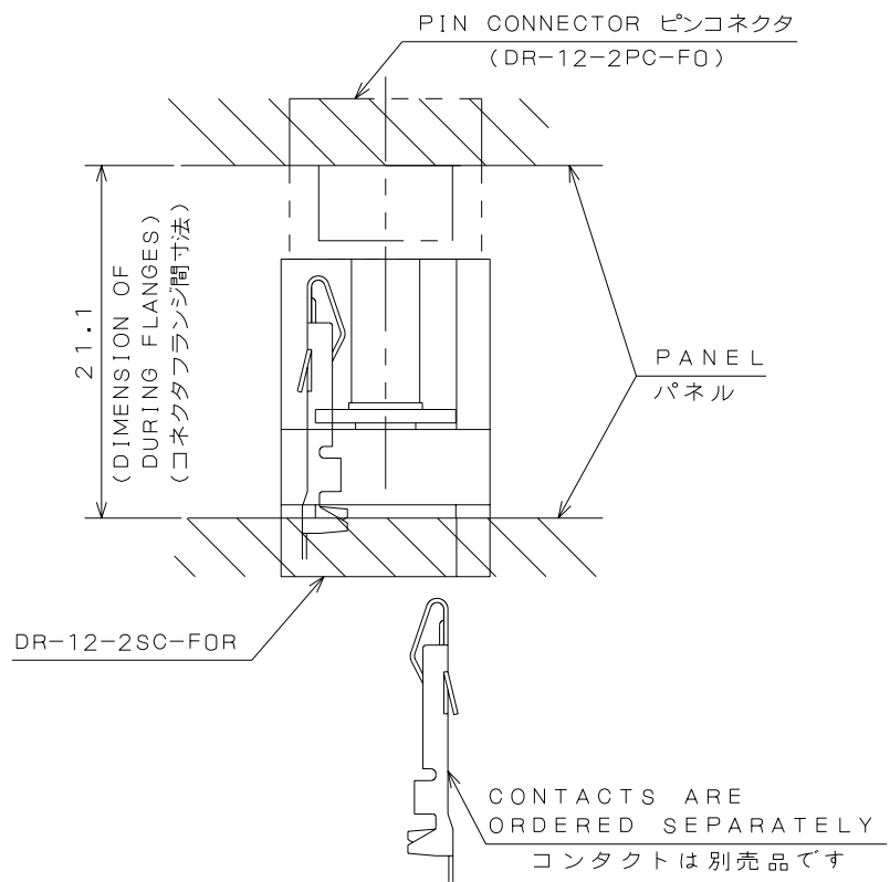
MATED CONDITION (REF.) 嵌合状態図 (参考)
