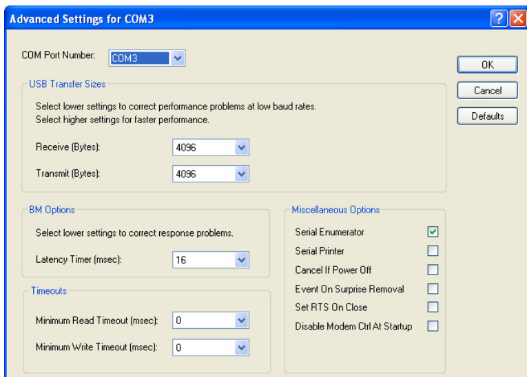
Figure 2.13 - Advanced Options
