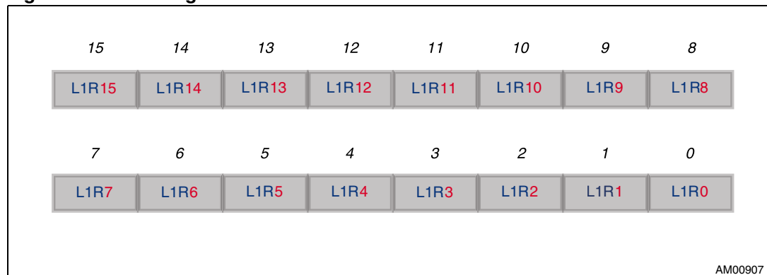
Figure 16. LED1 registers
