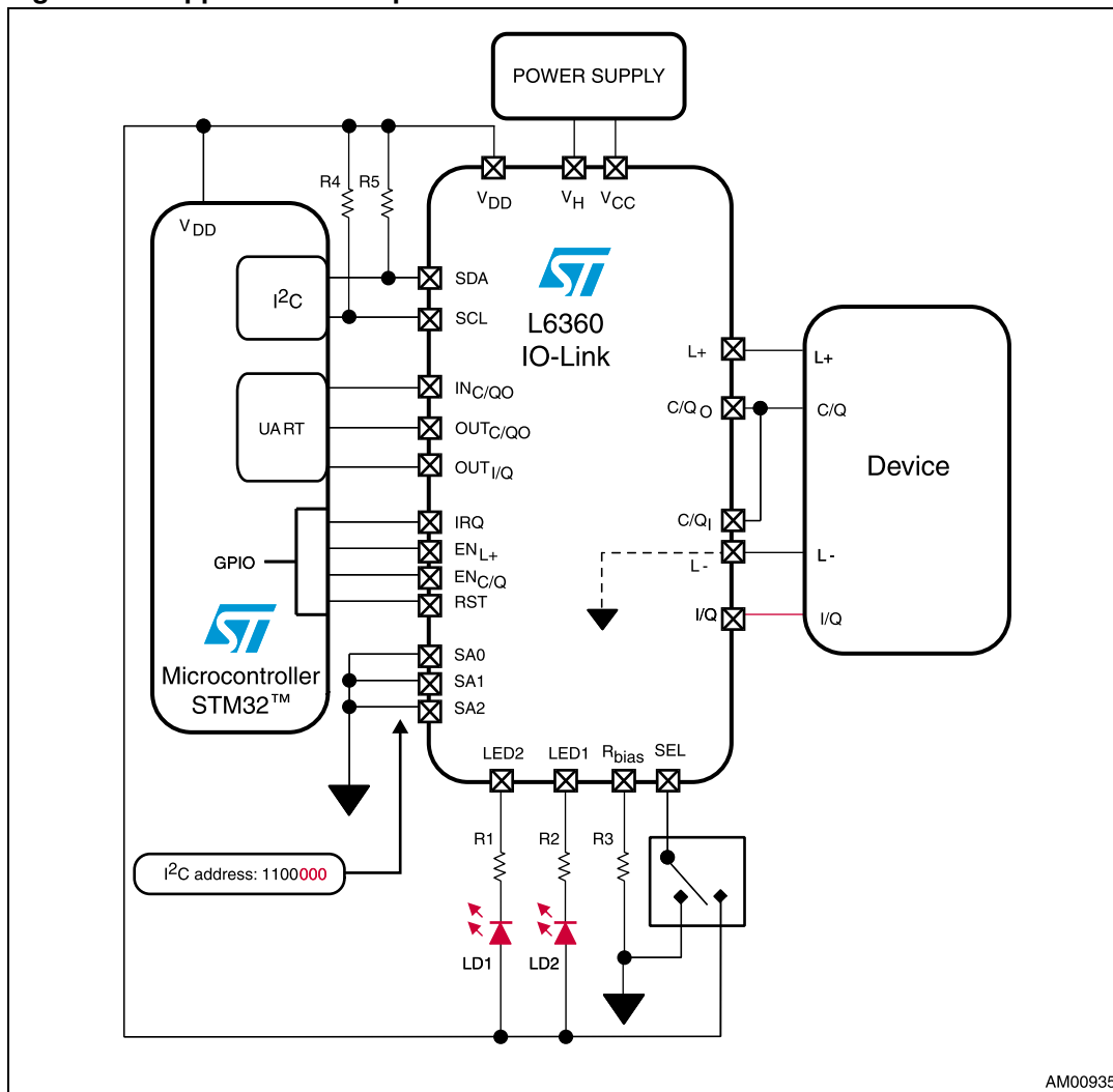
Figure 43. Application example
