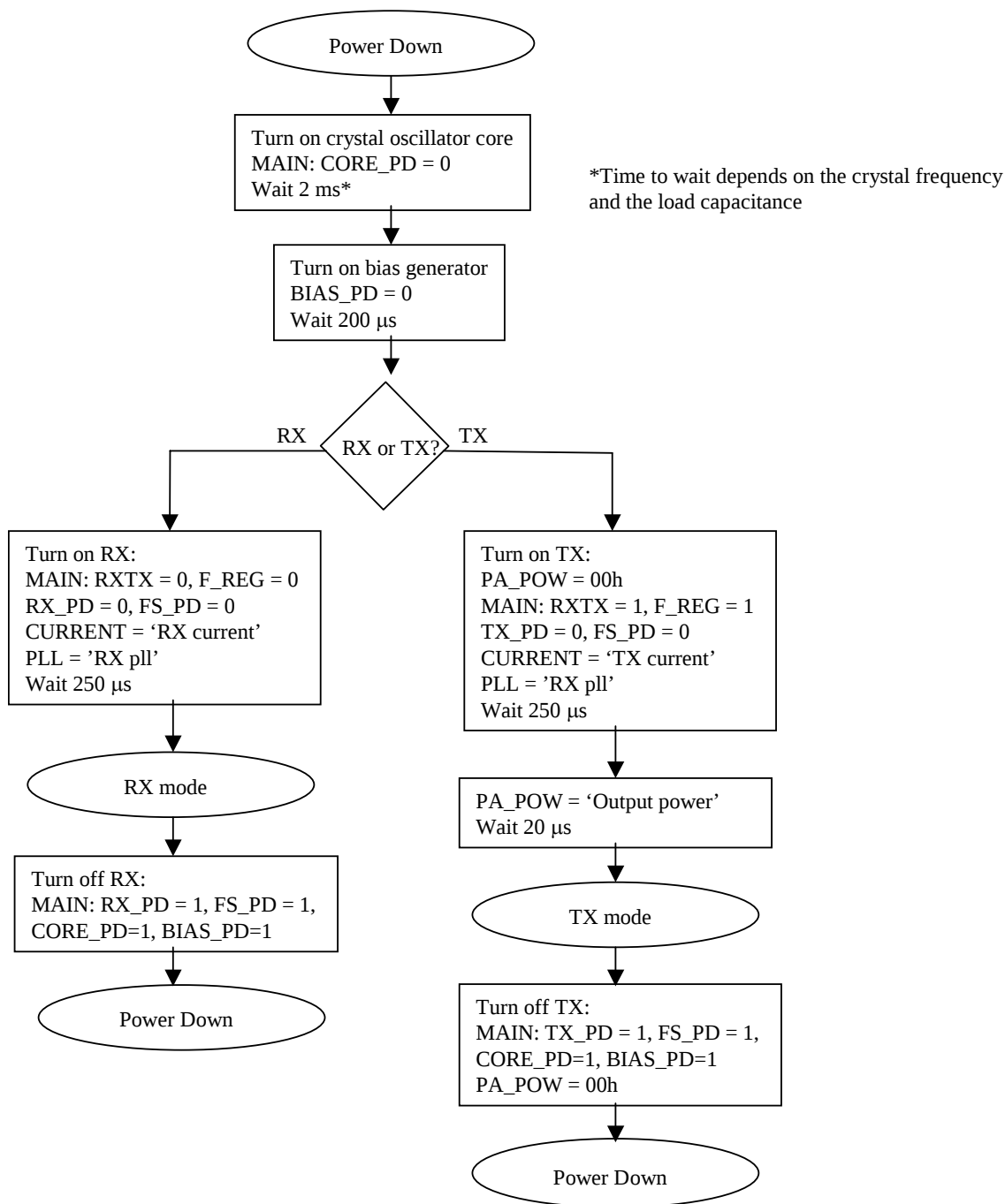
Figure 19. Sequence for activating RX or TX mode
