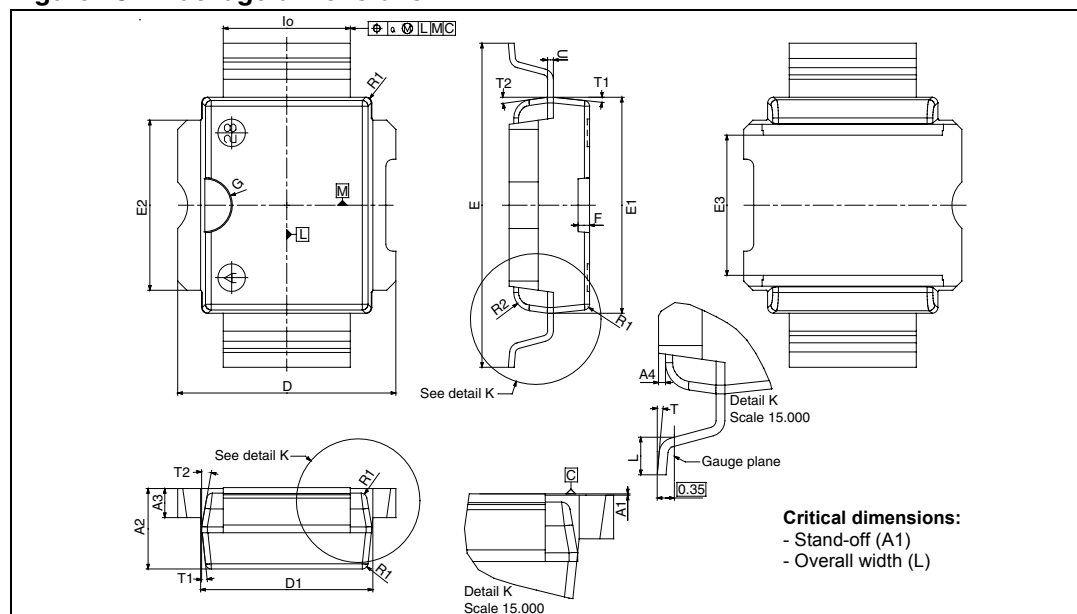
Figure 18. Package dimensions
